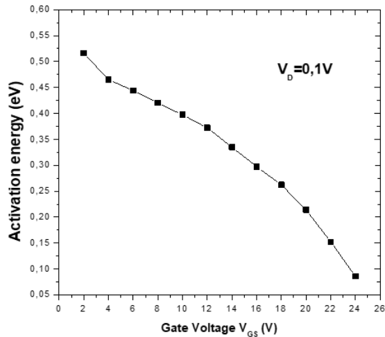
Figure 4. The evaluated activation energy versus the gate voltage
