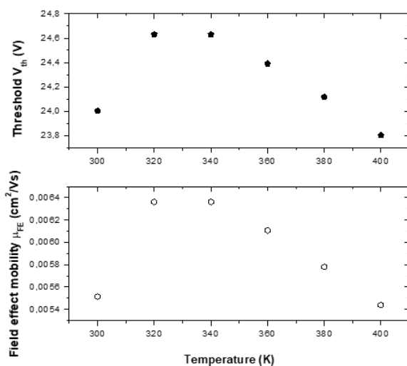
Figure 5. The effect of temperature on the field effect mobility and the threshold voltage extracted from the transfer characteristics I_D = f(V_{GS}) of the pc-ZnO TFT of figure 2.
