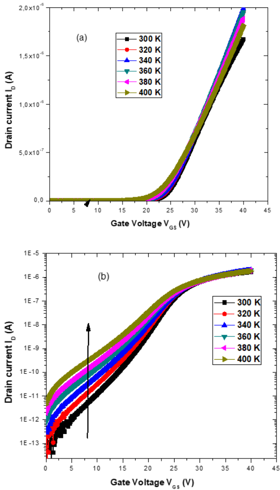
Figure 2: The simulated transfer characteristics I_D=f(V_{GS}) of the TFT for different temperatures ranging from 300 to 400 K on linear (a) and logarithmic (b) scales.
