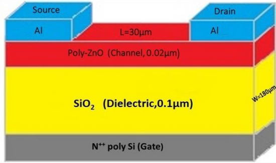
Figure 1: A three dimensional view of the pc-ZnO
