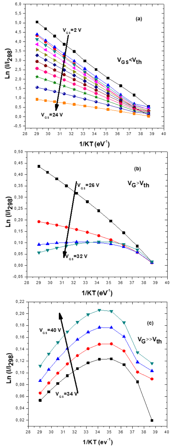
Figure 3. The Arrhenius plot of the normalized current I/I_{298} . (a) in the sub-threshold voltage, (b) just on the onset of the threshold voltage and (c) well beyond threshold voltage. I_{298} is the current at 298 K.
